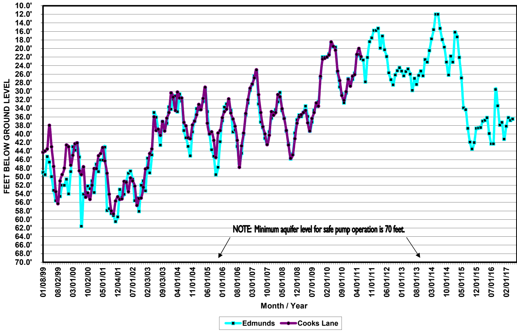
Towaco Valley Aquifer Water Levels
